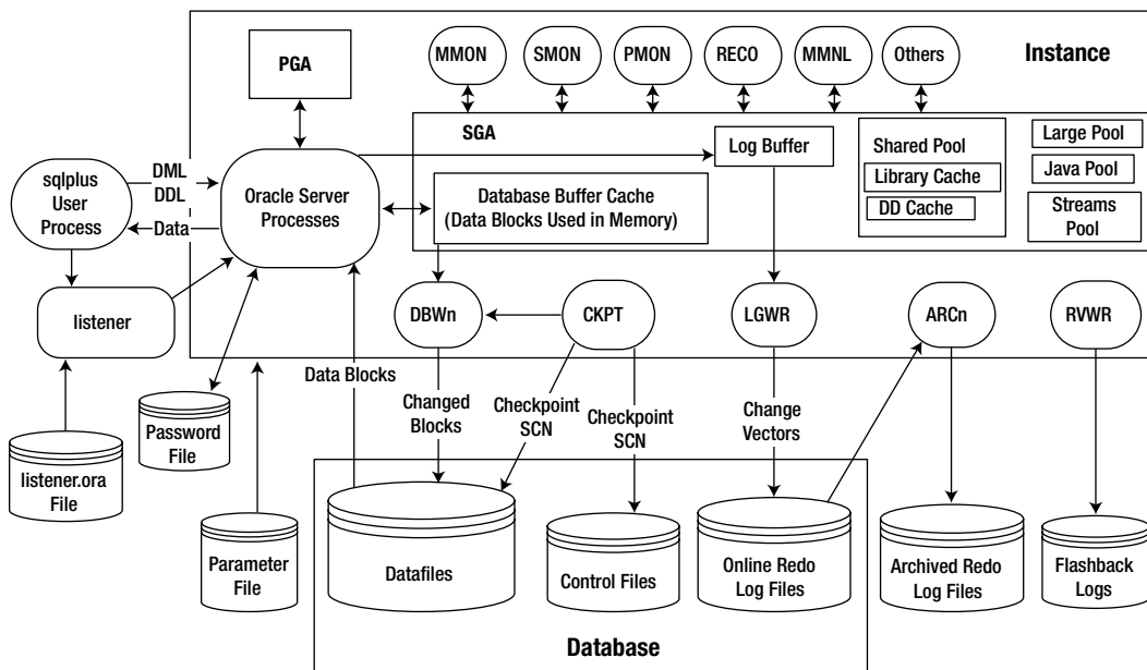
Figure 2-7. Oracle database architecture
