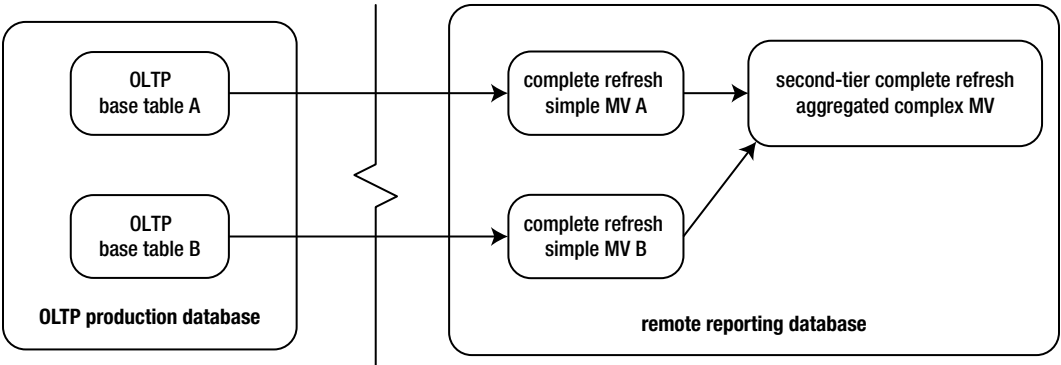
Figure 15-4. Remote refresh, using complete MV refreshes
