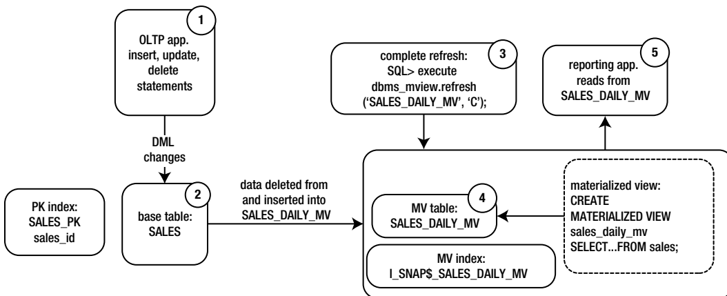
Figure 15-1. Architectural components of a complete refresh MV
