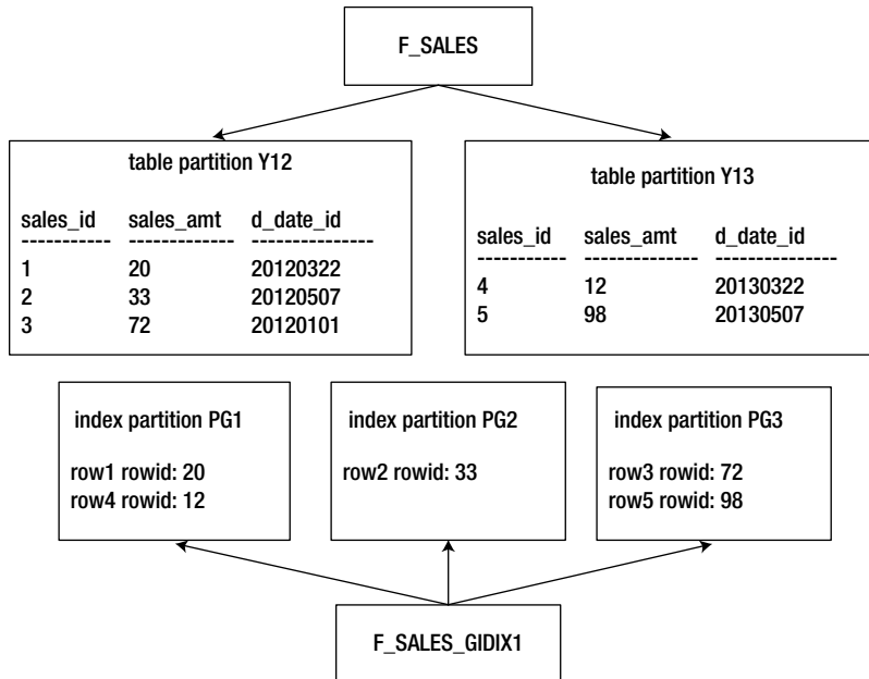
Figure 12-5. Architecture of a global index
